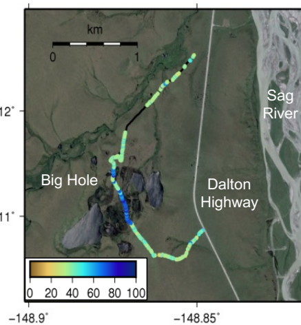
Figure 2: A sample GPR survey of ALT (cm) for the Big Hole wetland near Happy Valley airport on the North Slope of Alaska. Black indicates missing data.
